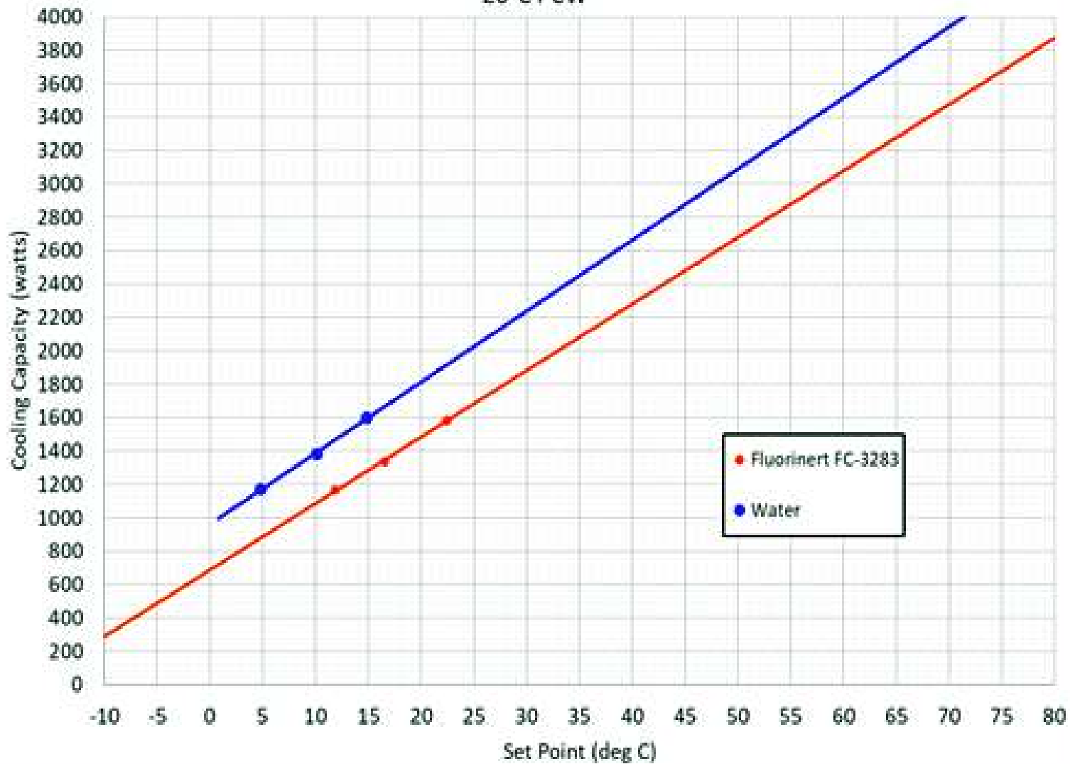
High Flow Thermorack 1801 Cooling Curves 20°C PCW
